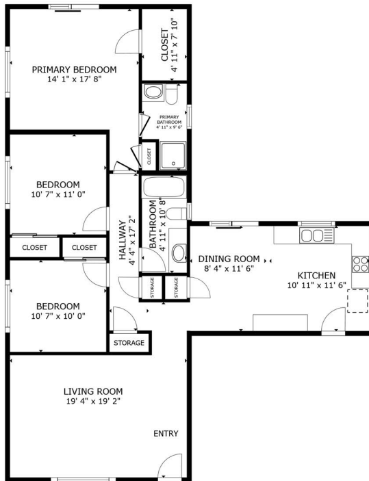
FLOOR PLAN
